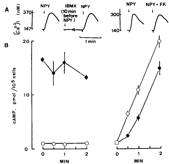
Fig.3. No implication of cyclic AMP in the NPY-induced [Ca^{2+}]_i rise. (A) Effect of forskolin and IBMX on NPY-induced increase in [Ca^{2+}]_i . Forskolin ( 10 \mu M , FK) was added simultaneously with NPY ( 10^{-6} M) and IBMX (0.1 mM) was added 10 min before NPY ( 10^{-6} M). Details as described in fig.1. (B) Effect of NPY stimulation on the cyclic AMP level in PASMC. (Left) Control (○—○) or IBMX-preincubated PASMC (●—●) were incubated with 10^{-6} M NPY. (Right) Incubations were initiated with the addition of 10 \mu M forskolin with (●—●) or without 10^{-6} M NPY (○—○). Cyclic AMP content was determined as described in section 2. Values are the mean \pm SE for 3 determinations.
